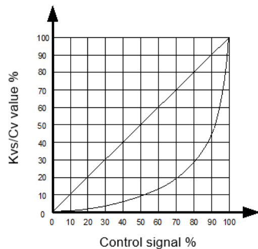
Fig. 14: Equal-percentage and linear characteristic
