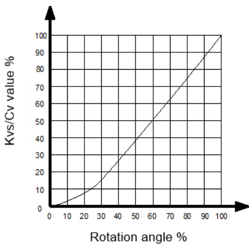
Fig. 13: Natural characteristic
