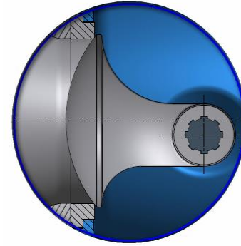
Fig. 11: Double-Eccentric Principle
