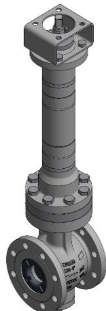
Fig. 2.7: Insulating section Type IT2
